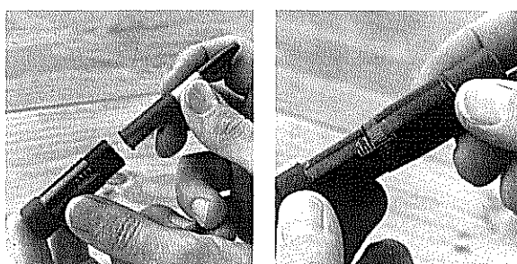
Insert the freebore tool into the body. Thread the land nut onto the body.
