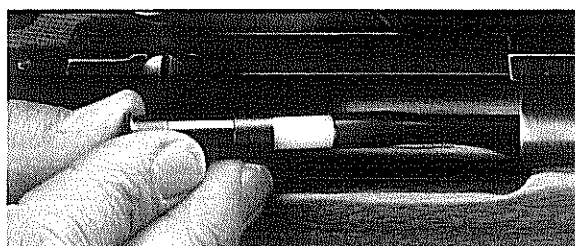
Chamber the freebore tool in the test rifle.
